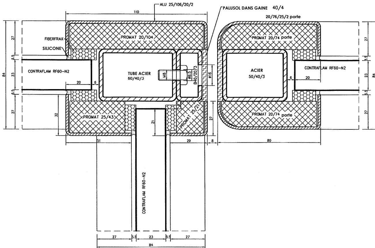
Figure 2 : Dimensions Contraflam 60 N2
